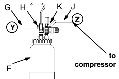
2-quart remote pressure pot
